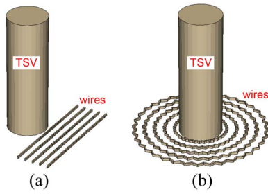
Fig. 7. Test structures for library generation. (a) Line library structure. (b) Ring library structure.
